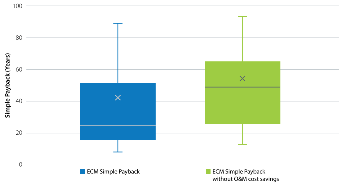
Figure 49. Distribution of GHP ECM simple payback as reported and with O&M cost savings removed.
