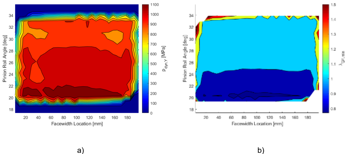
Figure 6 – a) Pressure distribution and b) specific film thickness across the contact zone for Case 2
