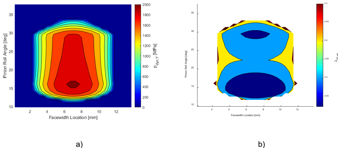
Figure 8 – a) Pressure distribution and b) specific film thickness across the contact zone for Case 3
