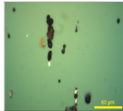
Photo 2: 500X shows normal rubbing, fatigue, spherical wear, and oxide particles at the entry region.
