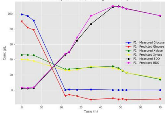
Fermenter 1 Experiment 25, Tracking Glucose, Xylose & BDO
