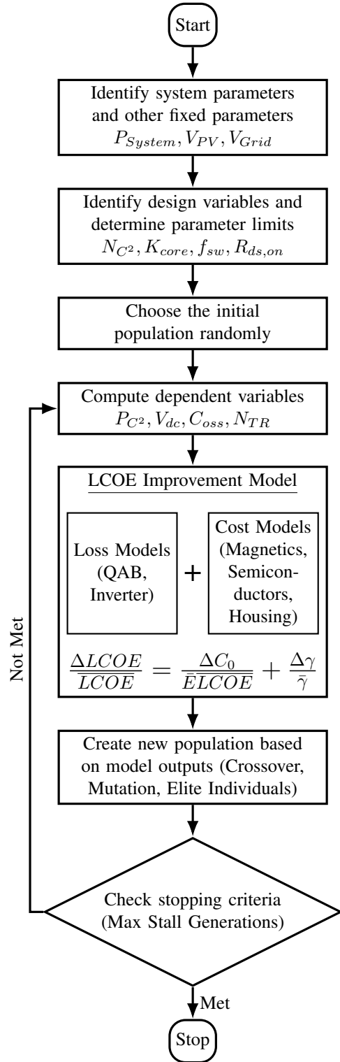
Fig. 2. Genetic Algorithm Flow Chart
