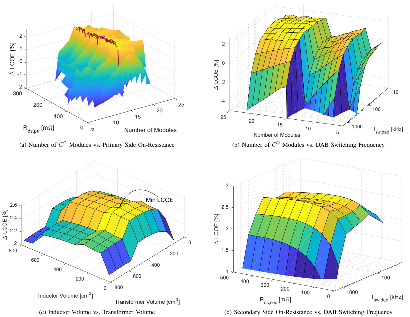
Fig. 3. Surface plots showing the relationships between various parameters and the LCOE improvement. The red line in (a) shows the path taken by the best design for each generation and the circles represent the best value for each generation. (a) is plotted with data from the genetic algorithm and (b) - (d) are plotted with sweeps around the optimal value to hold the variables not plotted constant.
