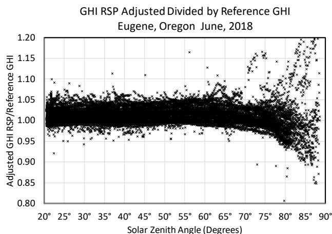
FIGURE 6. Ratio of adjusted RSP GHI and reference GHI obtained via the summation technique. It is only a large zenith angles (>75°) where difference start to appear.
